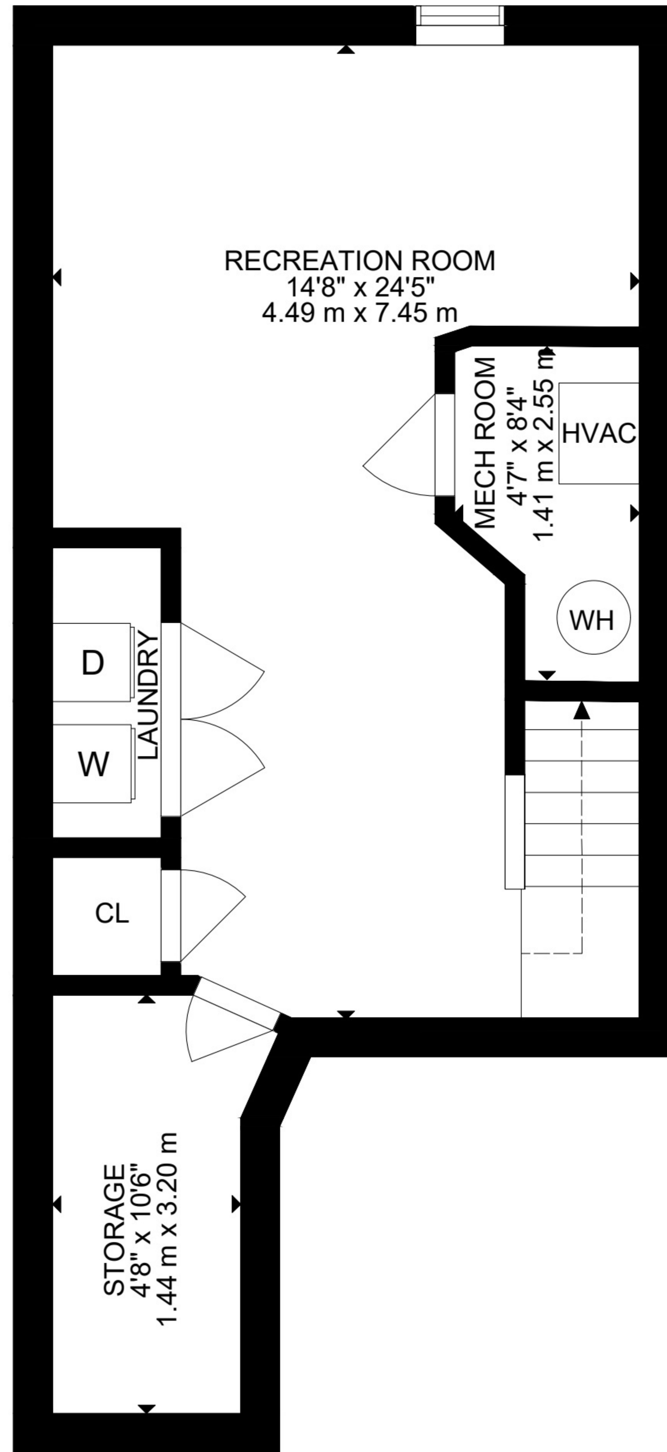
LOWER FLOOR
